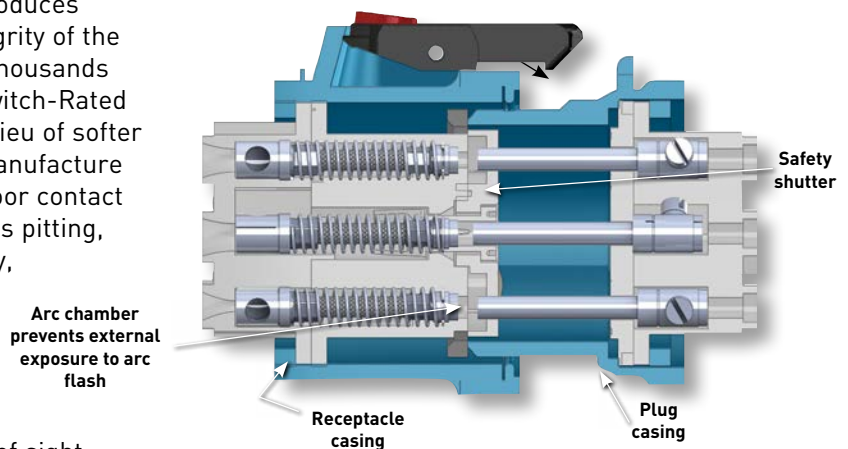
To obtain the functionality of a disconnect switch within a plug, MELTRIC Switch-Rated plugs are built with spring-loaded, butt-style contacts similar to those used on contactors and switchgear. This ensures that the integrity of the electrical connection is consistently maintained over thousands of operations.
