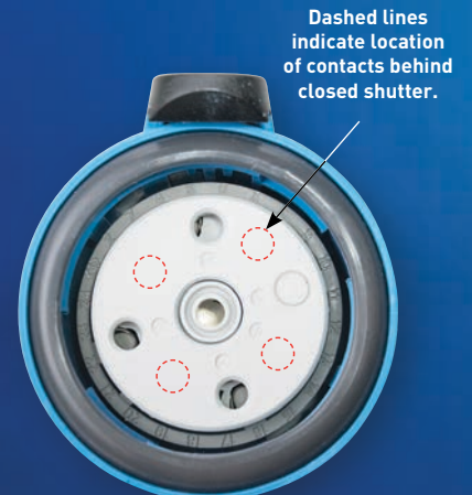
MELTRIC receptacle safety shutters block access to live contacts.
