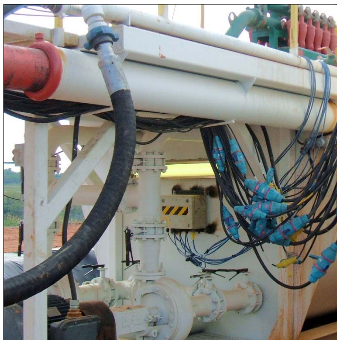
Pumps and other equipment benefit from Switch-Rated connections.
